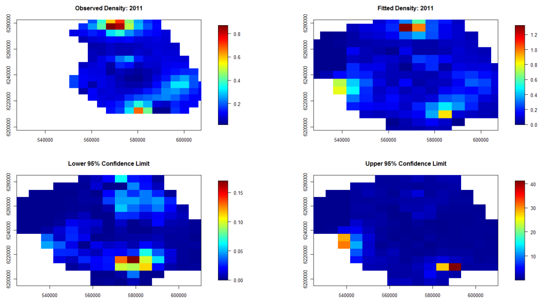
Figure 45: Estimated absolute densities per \text{km}^2 (i.e. with adjustment for availability) and upper and lower 95% confidence intervals for the densities (on a fine grid) in 2011 averaged in each grid cell.
