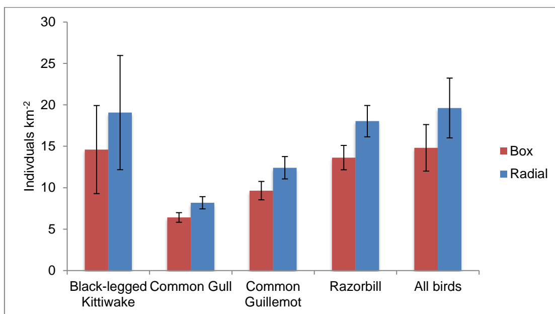
Figure 8. Mean density ( \pm 1 standard error) derived using the box and radial snapshot methods for the variety of medium-sized seabirds sampled as well as 'all birds' comprising a range of large to small species.
