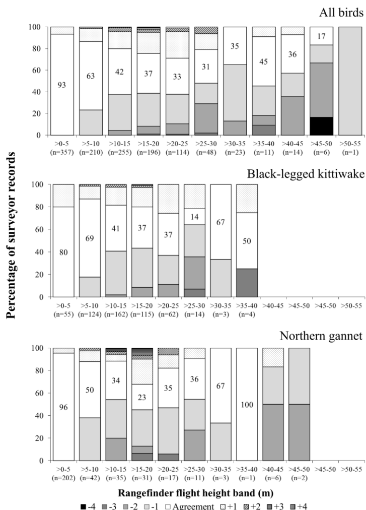
Figure 4. Variability in agreement (percentage of records) between range-finder and surveyor estimates of flight heights (in 5 m bands) for all birds (n=1,235), black-legged kittiwake (n=539) and northern gannet (n=350). Surveyor error is shown relative to under- and over-estimation by between 1 and 4 bands relative to the range-finder.
